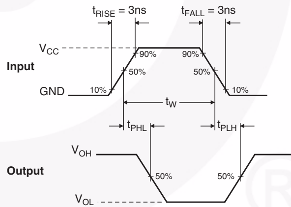
Figure 2. AC Waveforms
